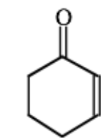
Cyclohexenone
