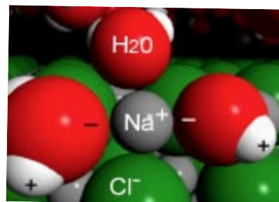
VisChem animation from depicting the hydration of a Na + ion on a NaCl surface.
