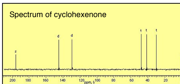
Cyclohexenone
